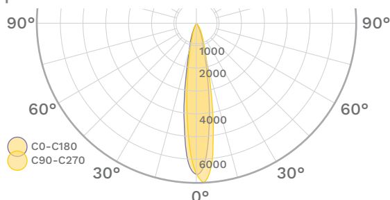
Aquila Surface 406.5mm 30°
