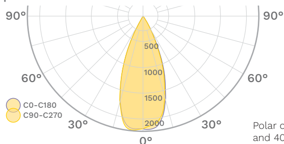
Aquila Surface 280mm 45°
