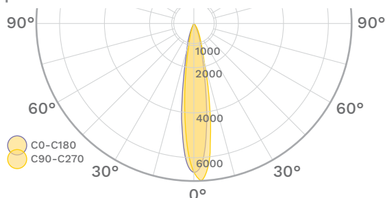
Aquila Surface 412mm 30°
