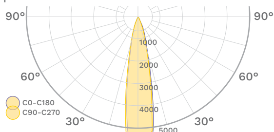
Aquila Surface 280mm 30°
