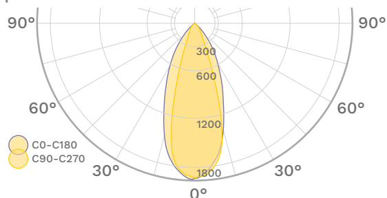
Aquila Surface 412mm 45°
