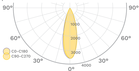
Aquila Surface 137mm 45°
