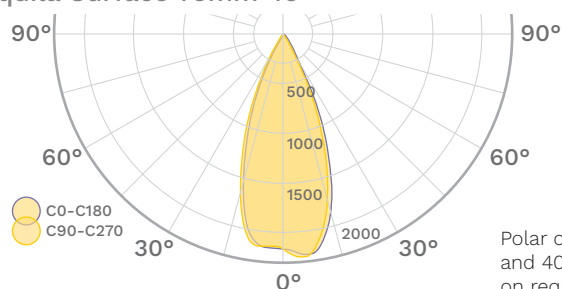
Aquila Surface 75mm 45°
