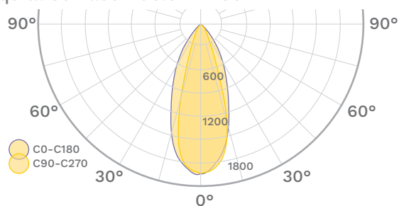
Aquila Surface 406.5mm 45°
