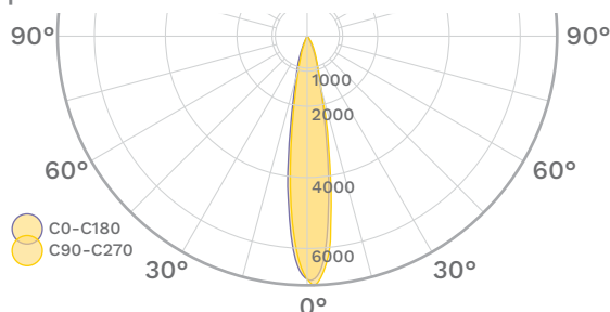
Aquila Surface 137mm 30°
