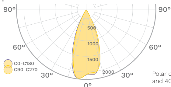
Aquila Surface 147mm 45°
