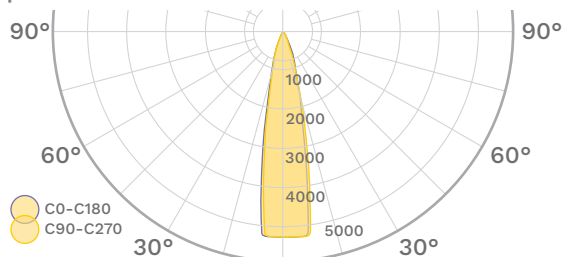
Aquila Surface 269.5mm 15°
