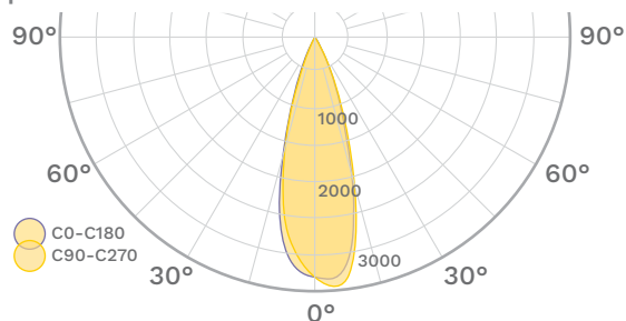
Aquila Surface 269.5mm 45°
