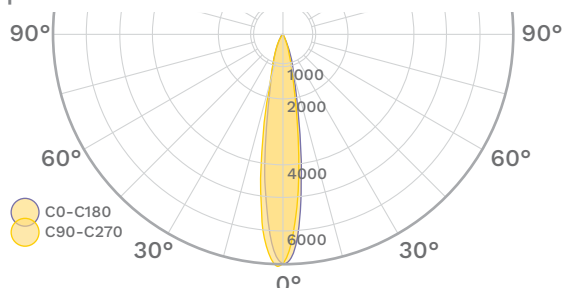
Aquila Surface 75mm 30°
