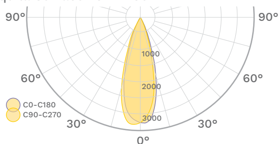
Aquila Surface 75mm 45°
