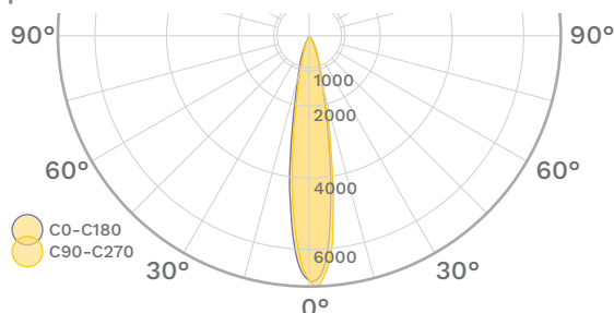
Aquila Surface 147mm 30°
